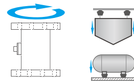
传感器受力图 Force diagram of sensor
