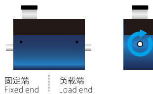
传感器受力图 Force diagram of sensor
